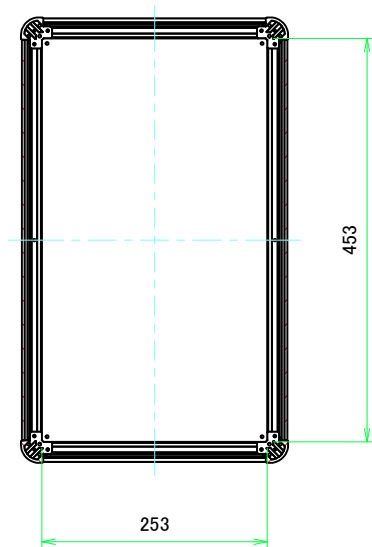
B-B (1:6)
