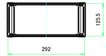
C-C (1:6)
