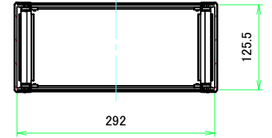
C-C (1:5.5)
