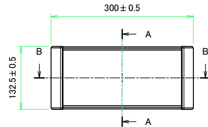
A view
