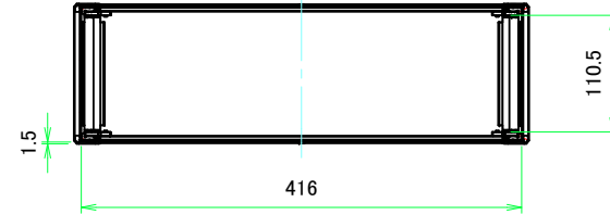
A-A (1:5.5)
