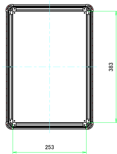
D view
