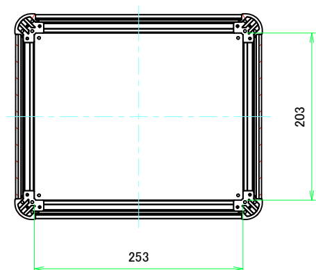
B-B (1:4.5)
