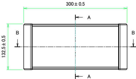
F view
