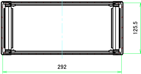
C-C (1:4)
