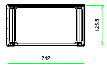
C-C (1:5)
