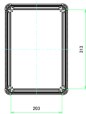
B-B (1:5)
