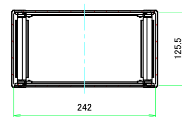
C-C (1:4.5)
