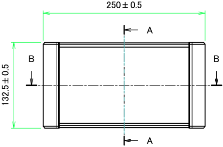
F view
