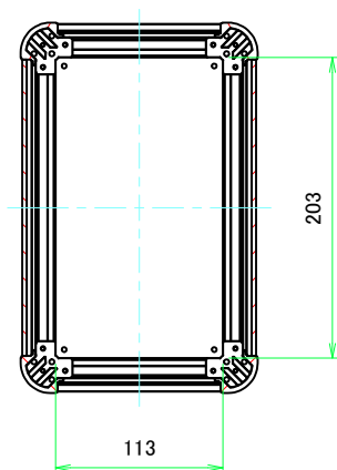
B-B (1:4)
