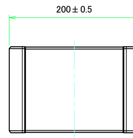
C view
