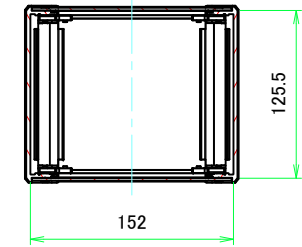
C-C (1:4)
