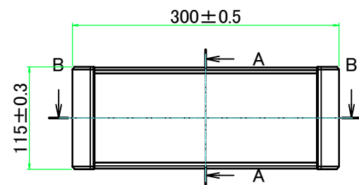
A view
