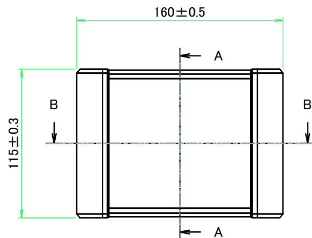
A view
