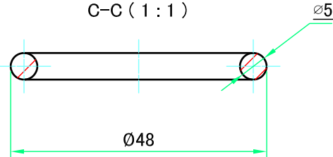
C-C (1:1)
